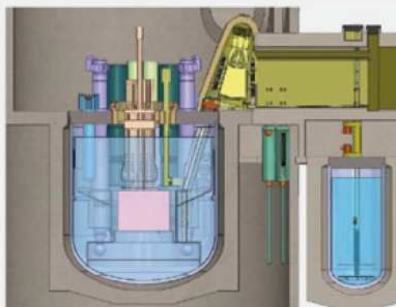
FIGURE 3.12: PRESENTATION OF THE FUEL ASSEMBLY HANDLING AND CLEANING SYSTEM
