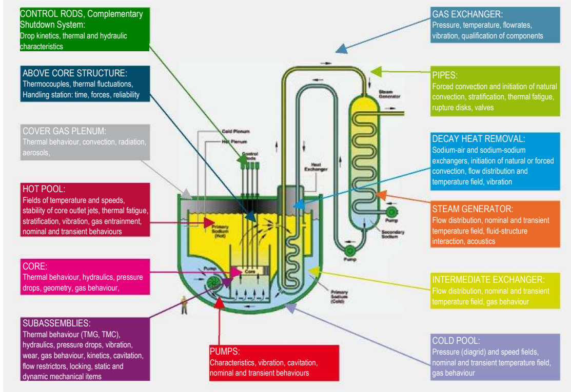
FIGURE 8.1: EXAMPLE OF PHENOMENA WHICH CAN BE STUDIED WITH SIMULATING FLUID MOCK-UPS
