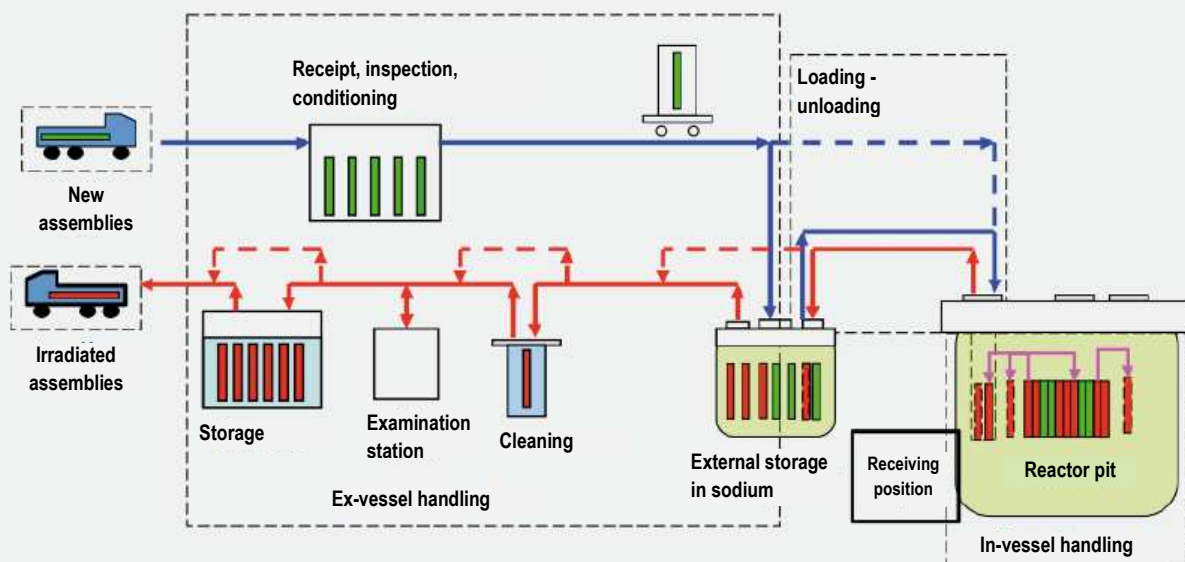
FIGURE 3.12: SCHEMATIC DIAGRAM OF THE FUEL HANDLING SYSTEM
