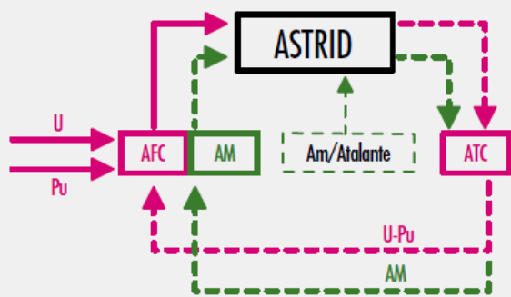
FIGURE 5.1: MATERIAL CYCLE FOR ASTRID
