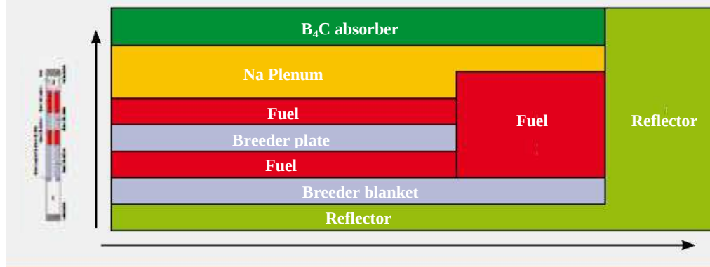
FIGURE 3: SCHEMATIC DIAGRAM OF THE FUEL PIN AND CFV CORE
