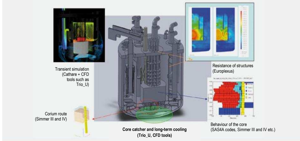
FIGURE 3.4: SEVERE ACCIDENTS AND ASSOCIATED MODELLING TOOLS
