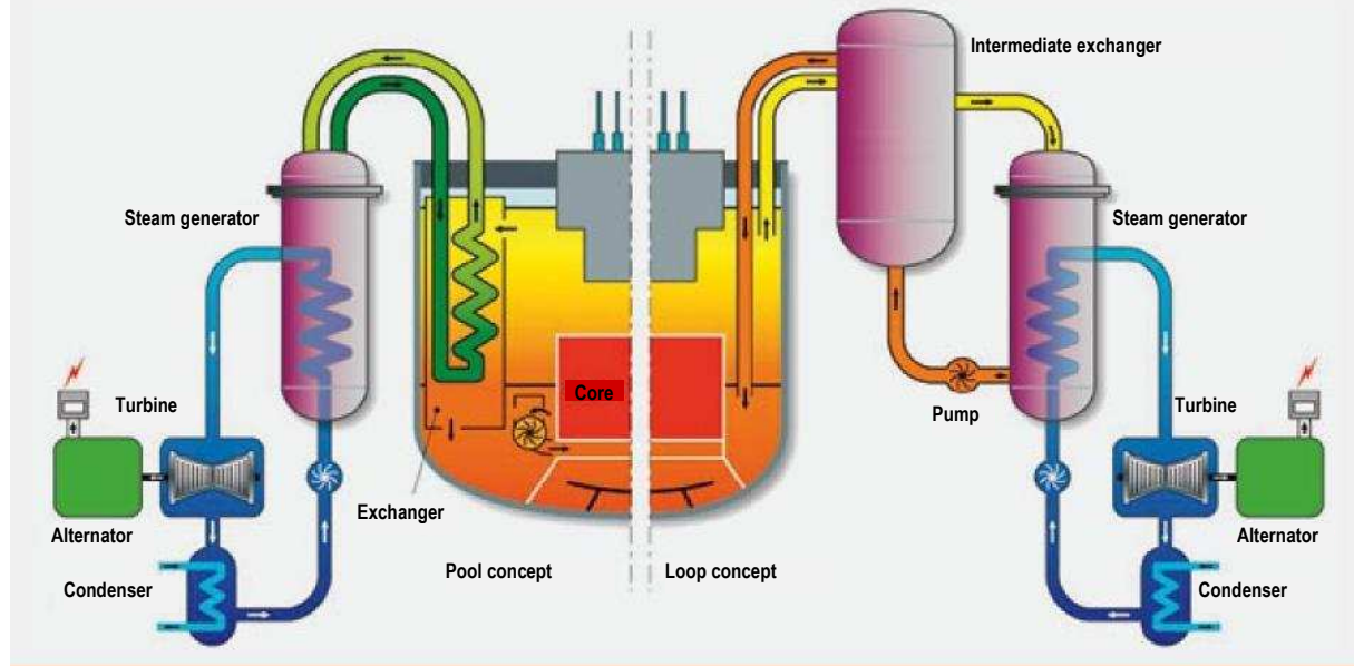
FIGURE A.2: ILLUSTRATION OF POOL AND LOOP CONCEPTS
