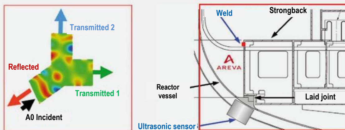
FIGURE 6.11: ULTRASONIC INSPECTION OF STRUCTURES
